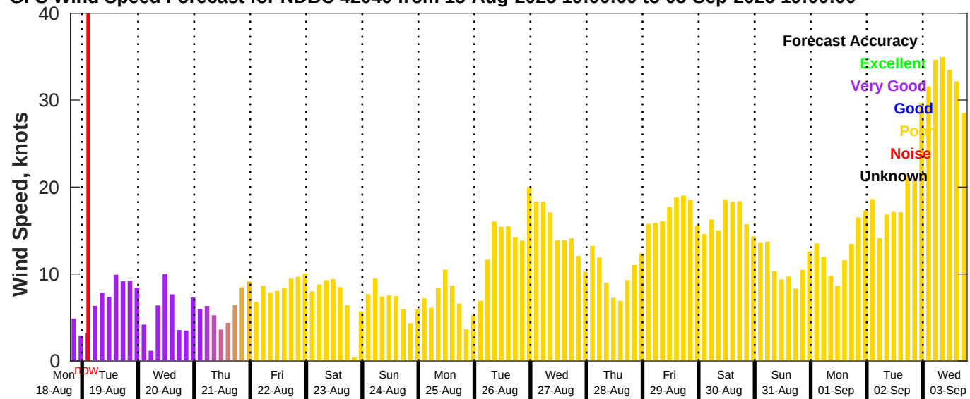
GFS Wind Speed Forecast for NDBC 42040 from 18-Aug-2025 19:00:00 to 03-Sep-2025 19:00:00
