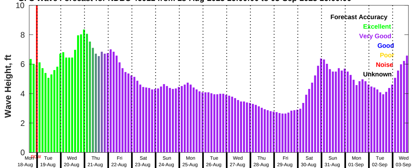
GFS Wave Forecast for NDBC 46011 from 18-Aug-2025 16:00:00 to 03-Sep-2025 16:00:00
