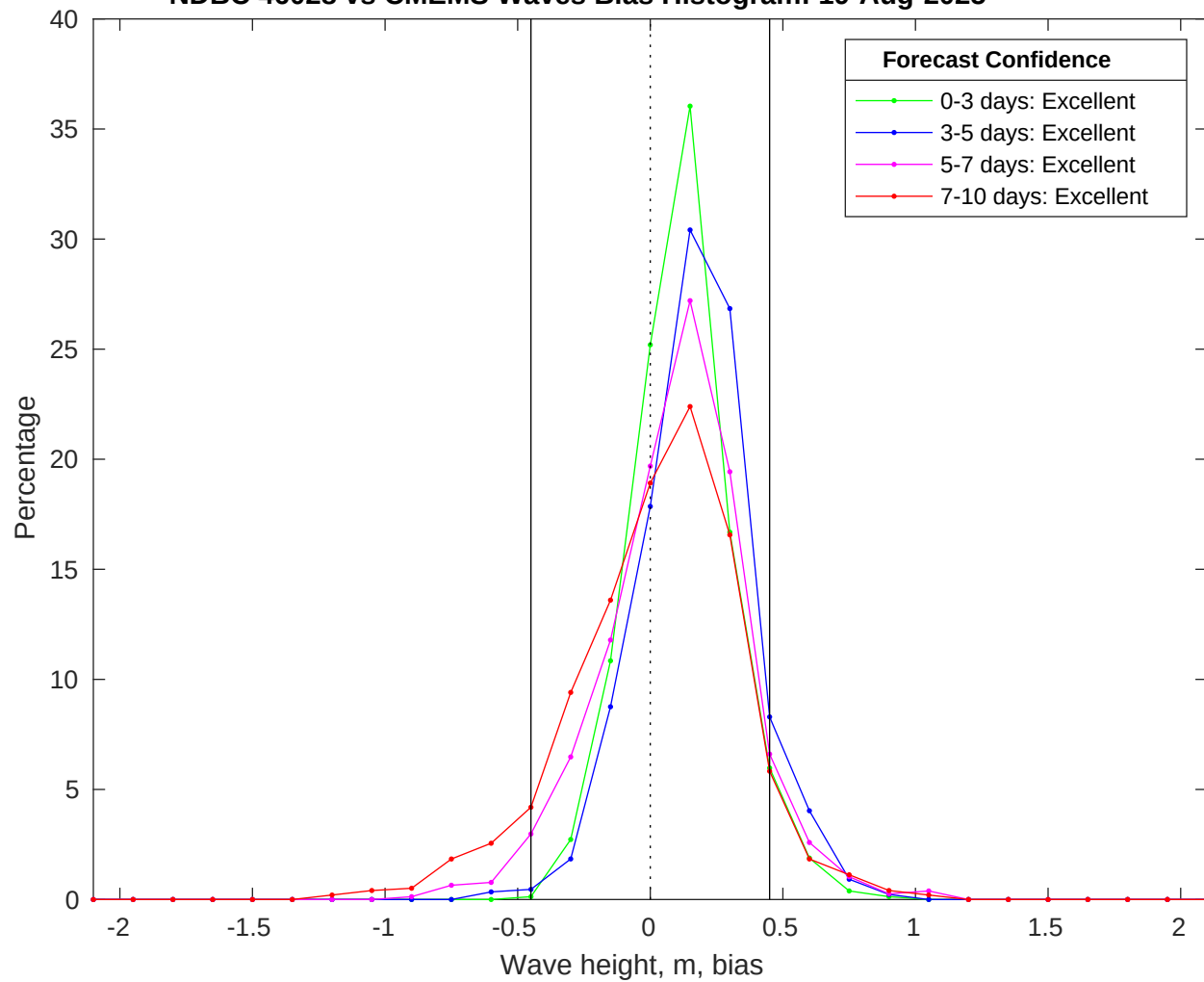
NDBC 46028 vs CMEMS Waves Bias Histogram: 19-Aug-2025
