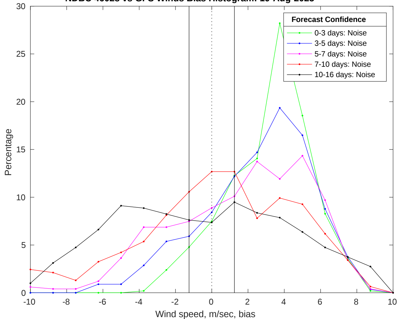
NDBC 46028 vs GFS Winds Bias Histogram: 19-Aug-2025
