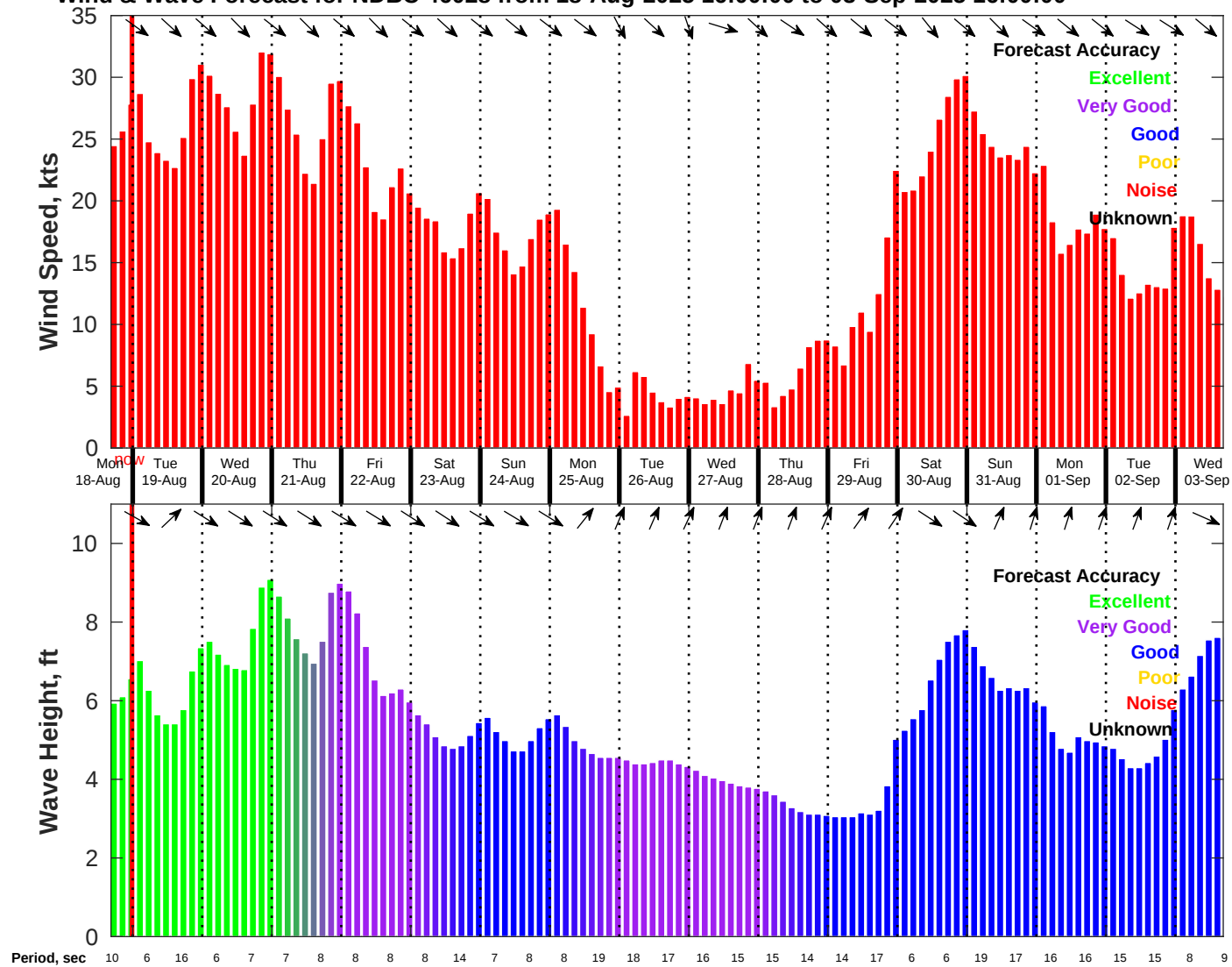
Wind & Wave Forecast for NDBC 46028 from 18-Aug-2025 16:00:00 to 03-Sep-2025 16:00:00
