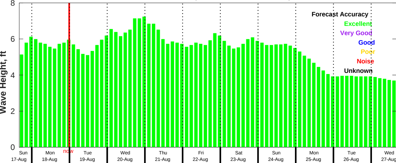
CMEMS Wave Forecast for NDBC 46054 from 17-Aug-2025 16:00:00 to 27-Aug-2025 16:00:00
