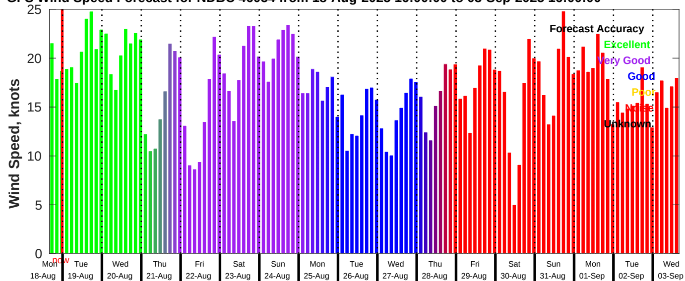
GFS Wind Speed Forecast for NDBC 46054 from 18-Aug-2025 16:00:00 to 03-Sep-2025 16:00:00
