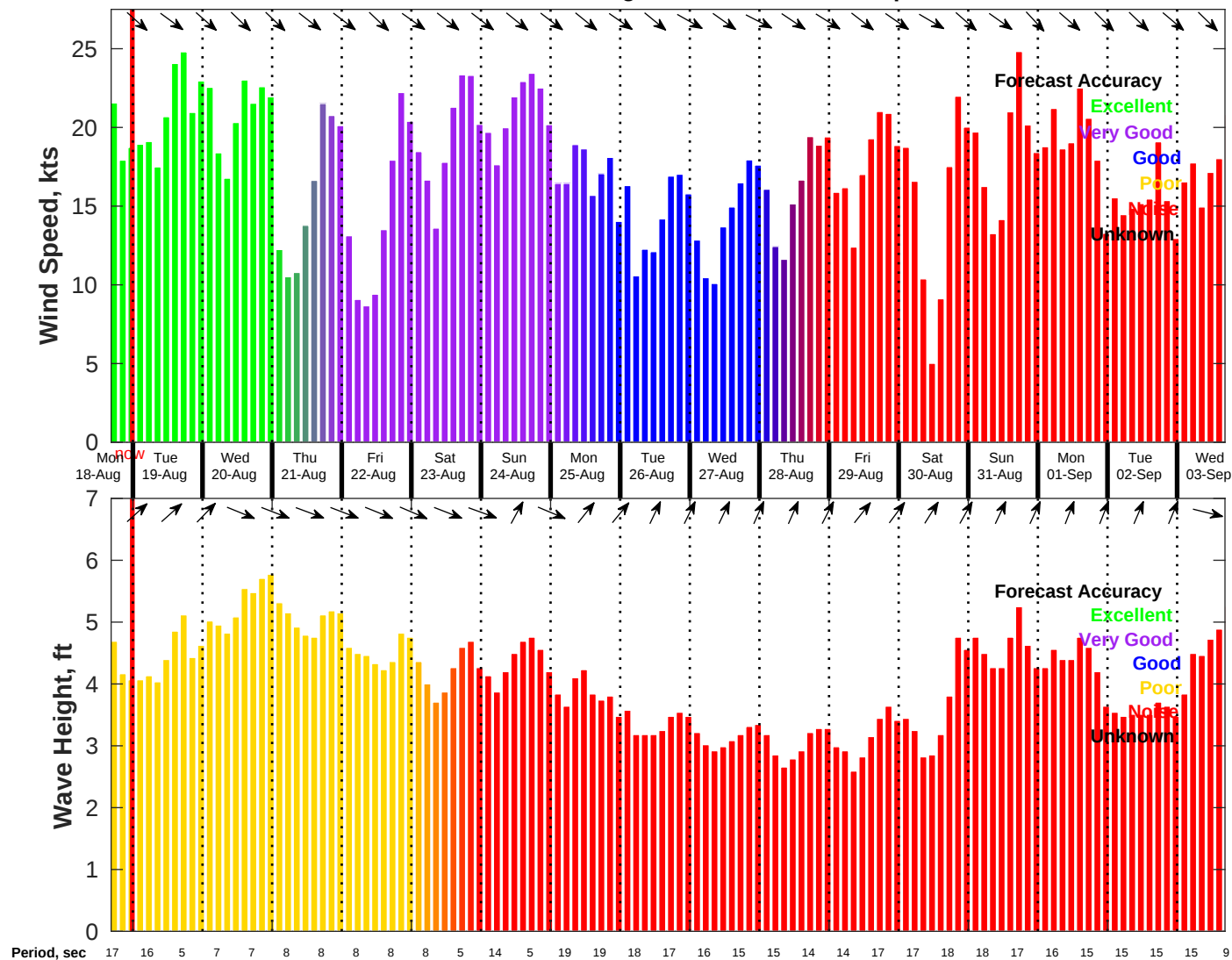
Wind & Wave Forecast for NDBC 46054 from 18-Aug-2025 16:00:00 to 03-Sep-2025 16:00:00
