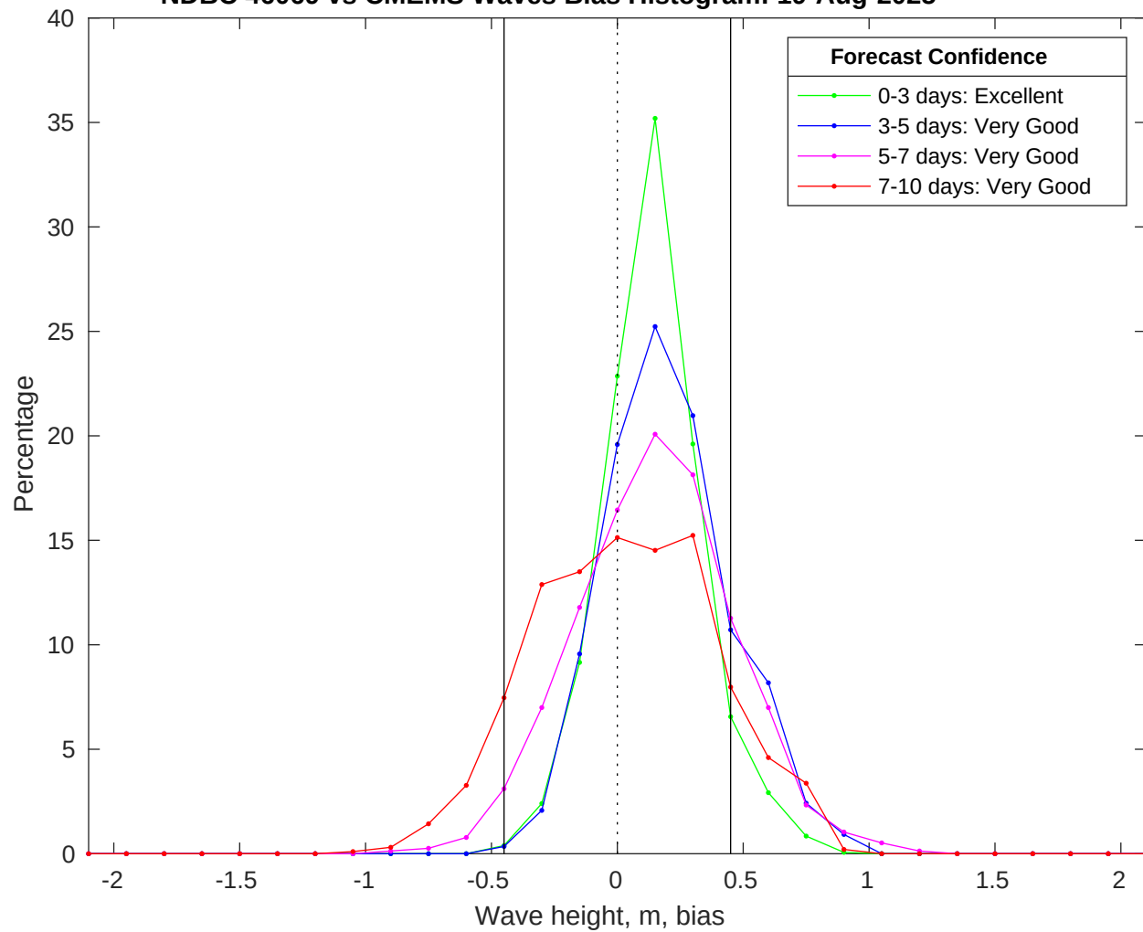
NDBC 46069 vs CMEMS Waves Bias Histogram: 19-Aug-2025
