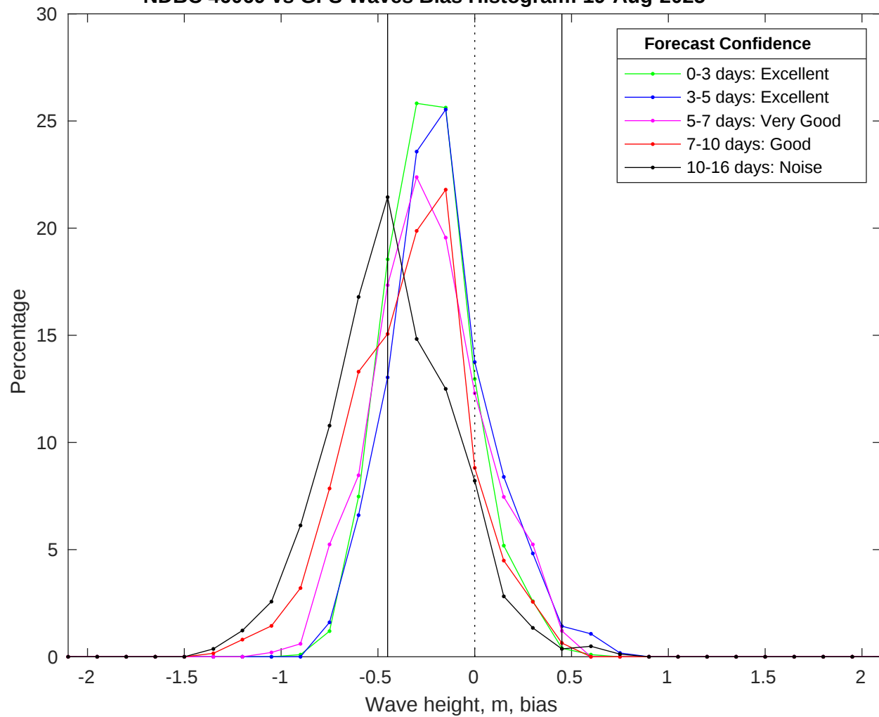
NDBC 46069 vs GFS Waves Bias Histogram: 19-Aug-2025
