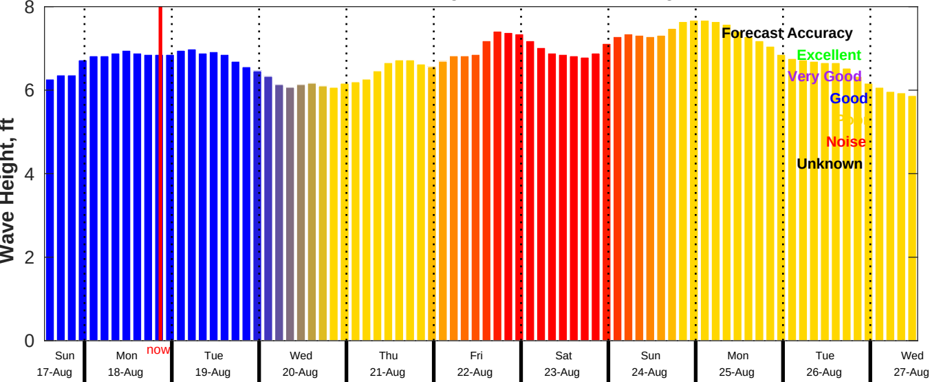
CMEMS Wave Forecast for NDBC 51209 from 17-Aug-2025 13:00:00 to 27-Aug-2025 13:00:00
