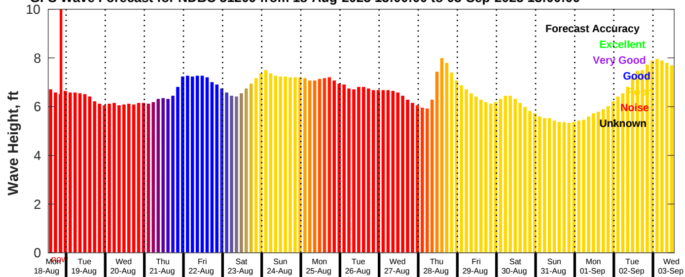
GFS Wave Forecast for NDBC 51209 from 18-Aug-2025 13:00:00 to 03-Sep-2025 13:00:00
