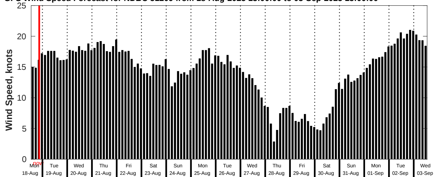
GFS Wind Speed Forecast for NDBC 51209 from 18-Aug-2025 13:00:00 to 03-Sep-2025 13:00:00
