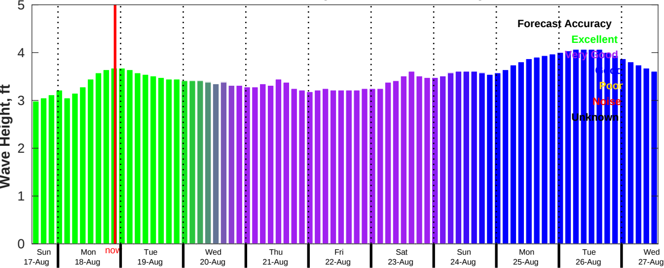
CMEMS Wave Forecast for NDBC 51211 from 17-Aug-2025 14:00:00 to 27-Aug-2025 14:00:00
