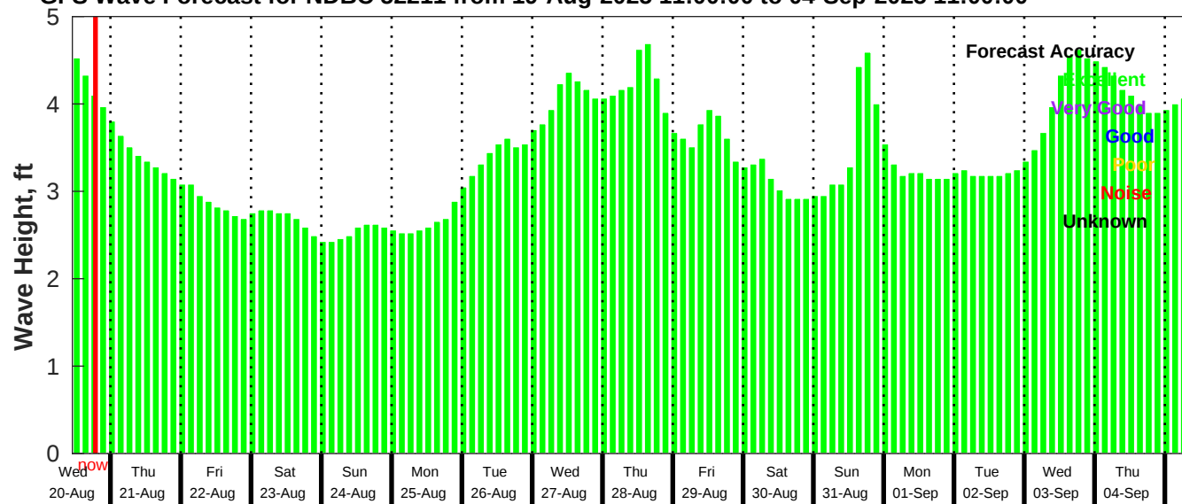
GFS Wave Forecast for NDBC 52211 from 19-Aug-2025 11:00:00 to 04-Sep-2025 11:00:00
