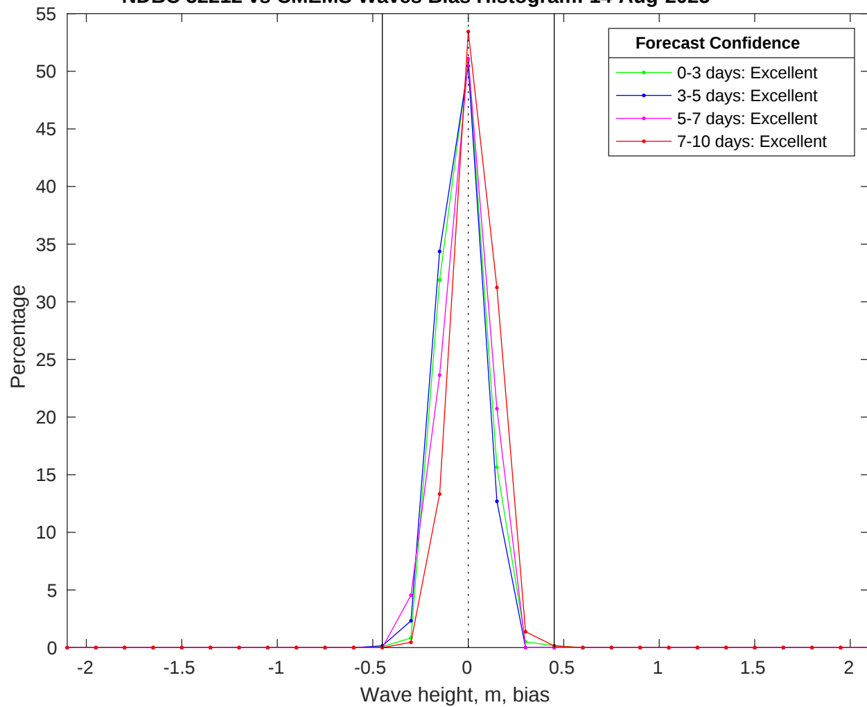
NDBC 52212 vs CMEMS Waves Bias Histogram: 14-Aug-2025
