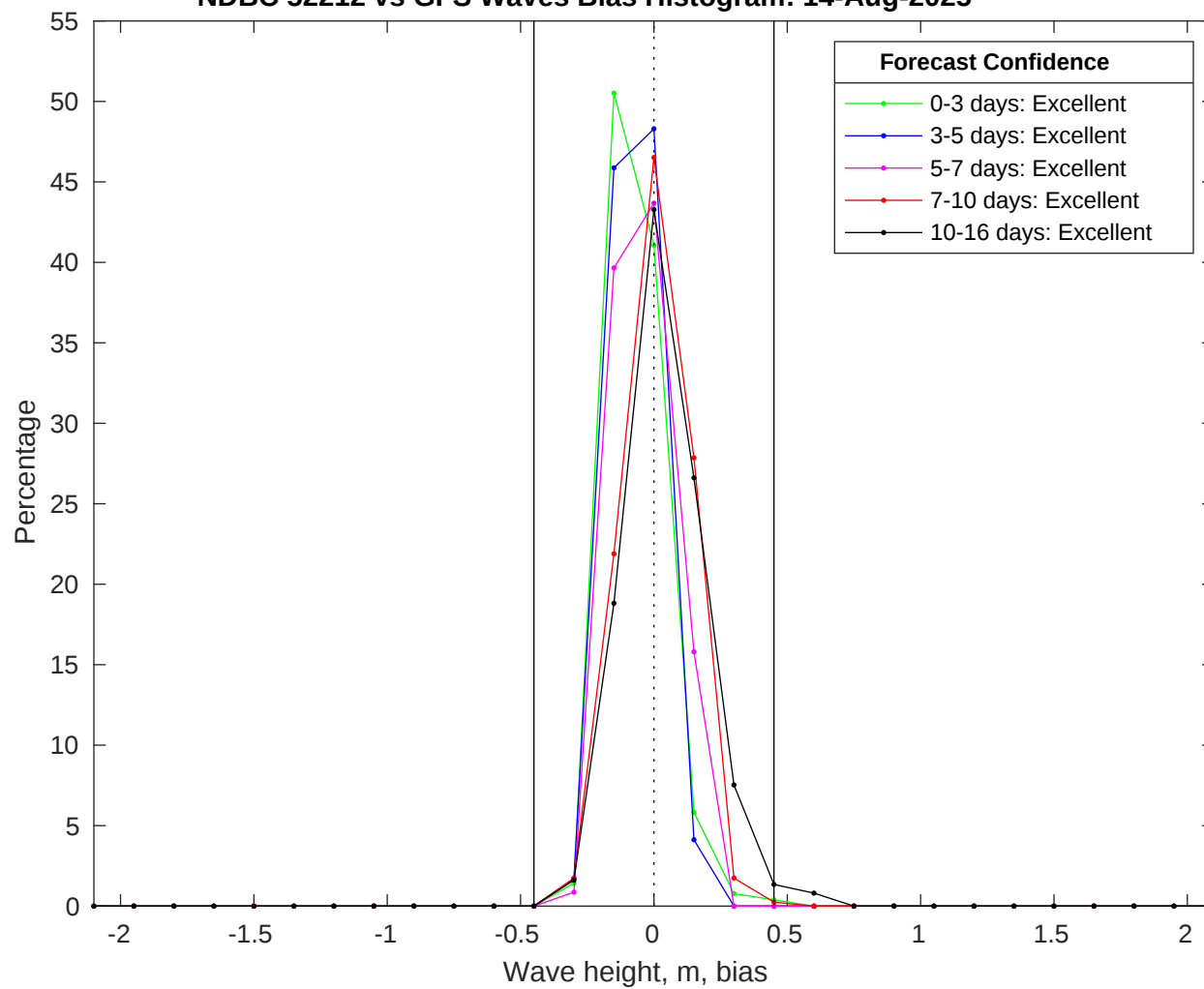
NDBC 52212 vs GFS Waves Bias Histogram: 14-Aug-2025
