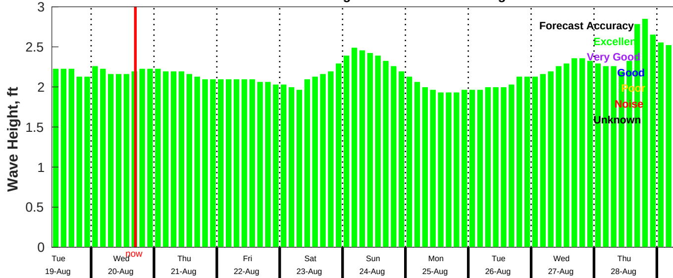
CMEMS Wave Forecast for NDBC 52212 from 18-Aug-2025 09:00:00 to 28-Aug-2025 09:00:00
