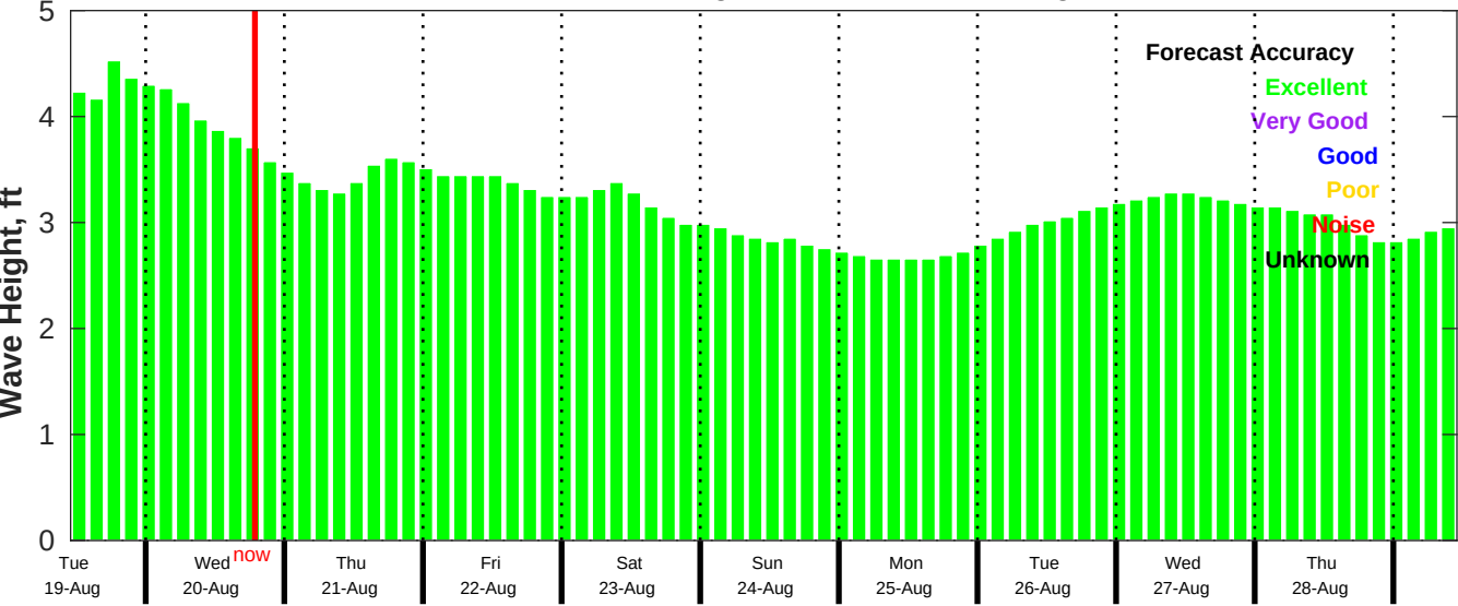
CMEMS Wave Forecast for NDBC 52213 from 18-Aug-2025 11:00:00 to 28-Aug-2025 11:00:00
