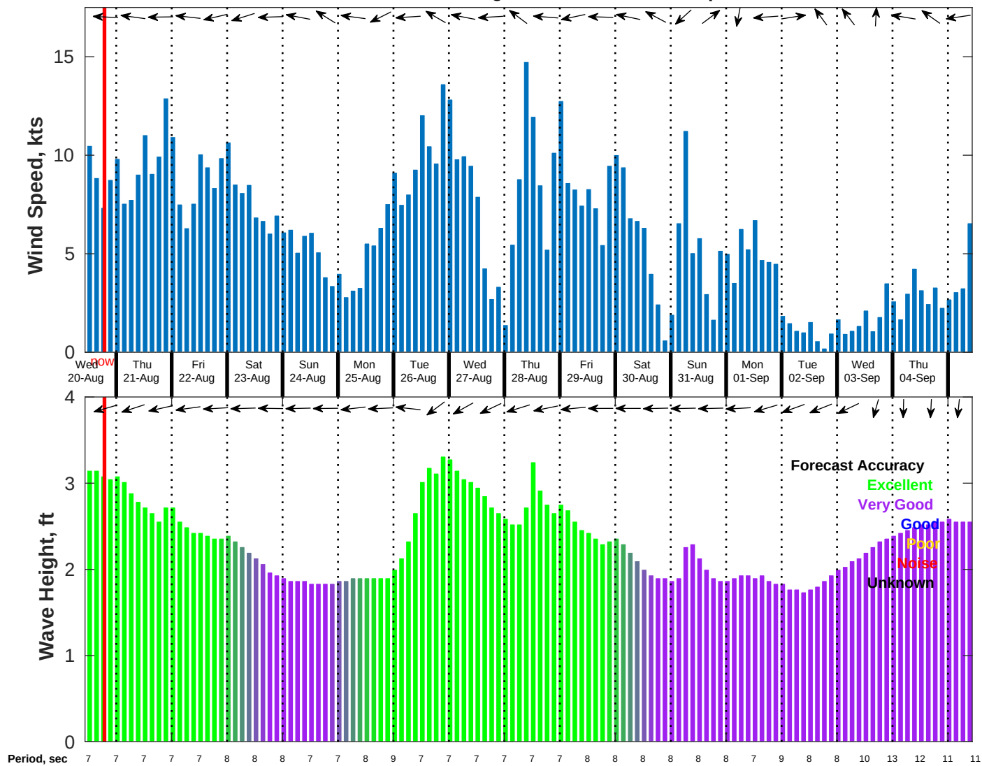
Wind & Wave Forecast for NDBC 52213 from 19-Aug-2025 11:00:00 to 04-Sep-2025 11:00:00
