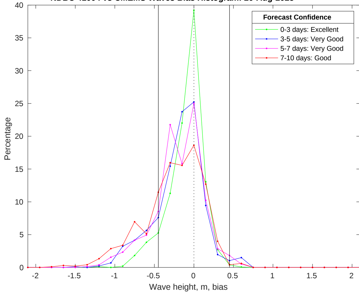
NDBC 41004 vs CMEMS Waves Bias Histogram: 20-Aug-2025
