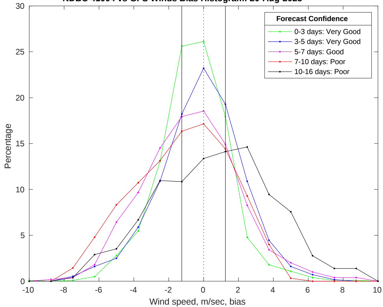
NDBC 41004 vs GFS Winds Bias Histogram: 20-Aug-2025
