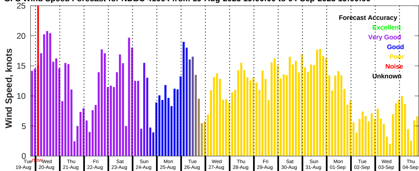
GFS Wind Speed Forecast for NDBC 41004 from 19-Aug-2025 19:00:00 to 04-Sep-2025 19:00:00
