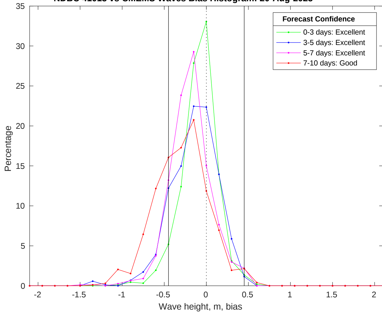
NDBC 41013 vs CMEMS Waves Bias Histogram: 20-Aug-2025
