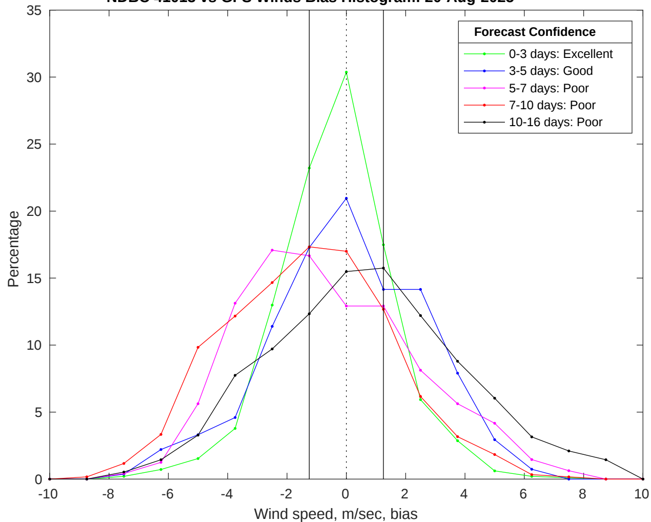
NDBC 41013 vs GFS Winds Bias Histogram: 20-Aug-2025
