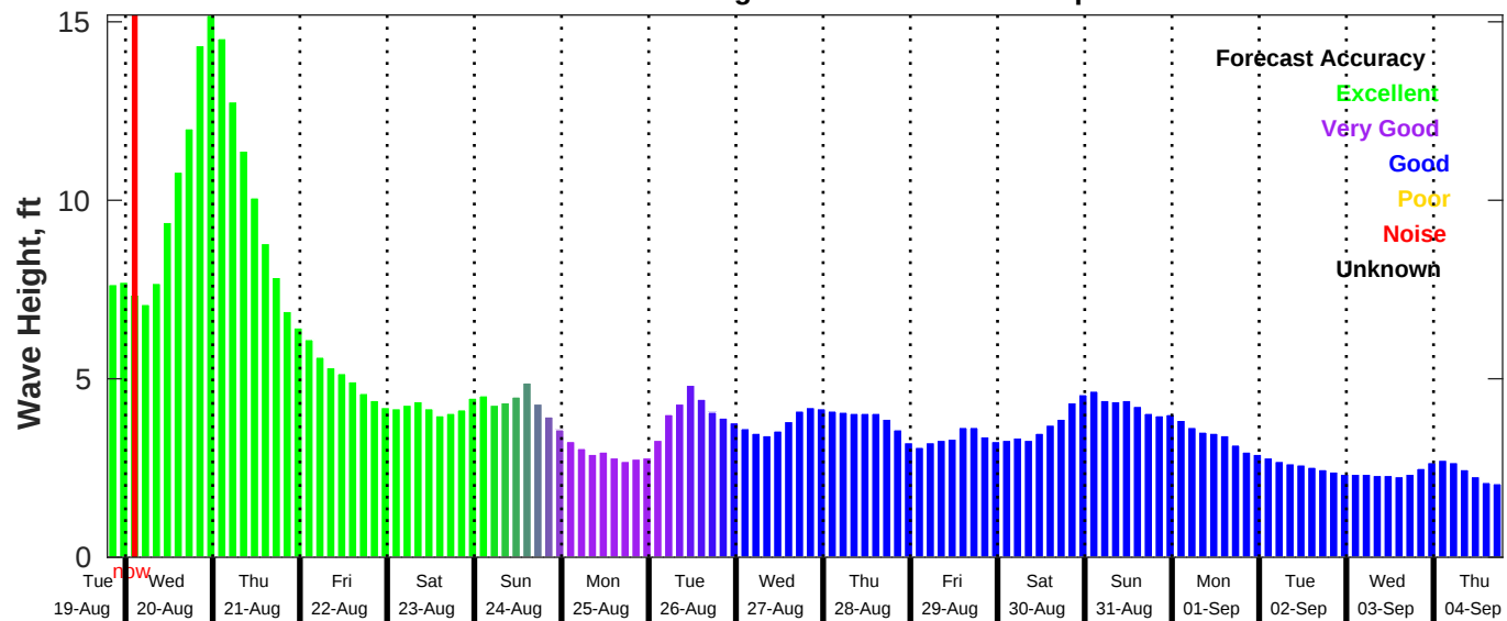
GFS Wave Forecast for NDBC 41013 from 19-Aug-2025 19:00:00 to 04-Sep-2025 19:00:00
