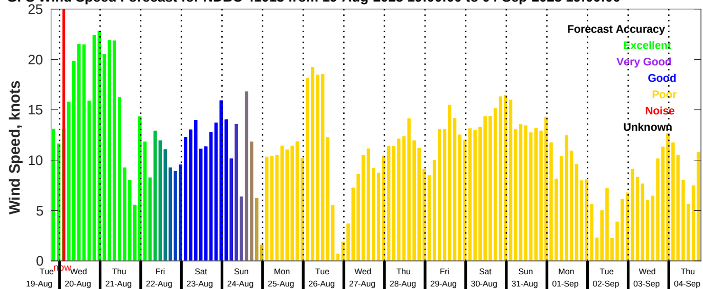
GFS Wind Speed Forecast for NDBC 41013 from 19-Aug-2025 19:00:00 to 04-Sep-2025 19:00:00
