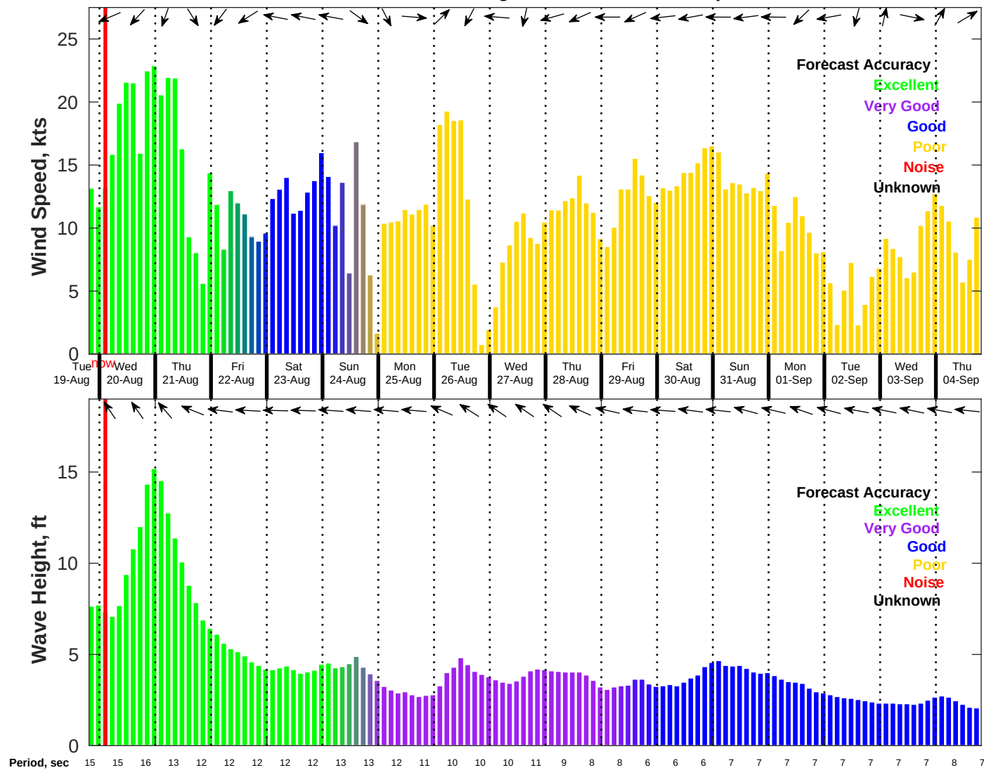
Wind & Wave Forecast for NDBC 41013 from 19-Aug-2025 19:00:00 to 04-Sep-2025 19:00:00
