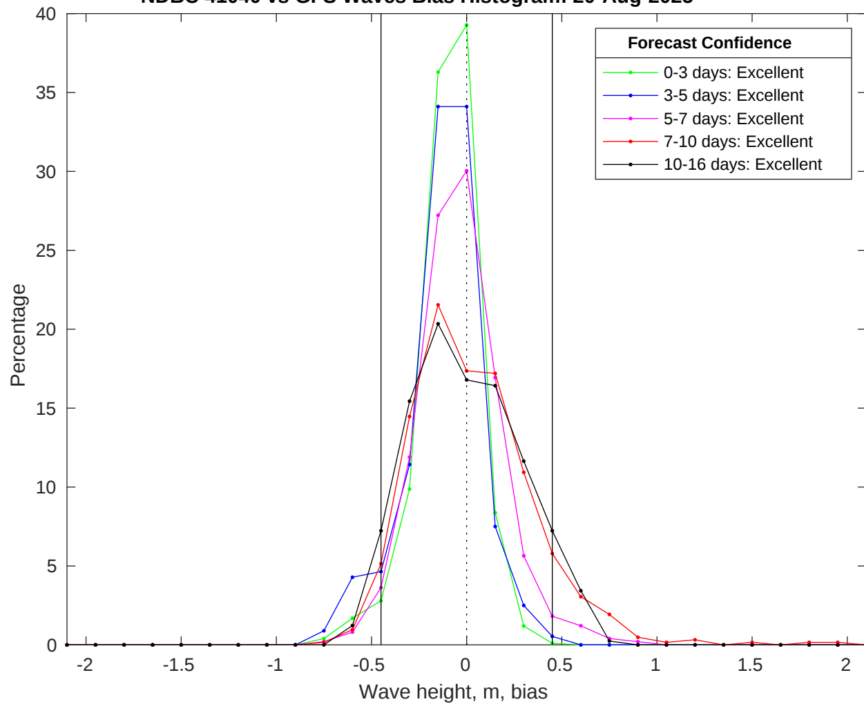
NDBC 41040 vs GFS Waves Bias Histogram: 20-Aug-2025
