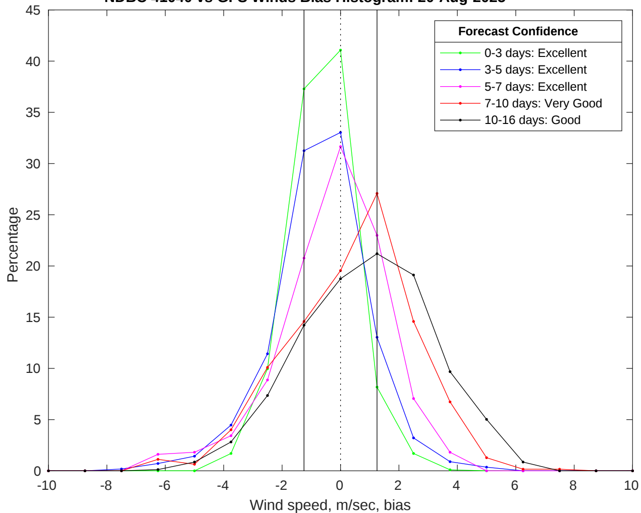
NDBC 41040 vs GFS Winds Bias Histogram: 20-Aug-2025
