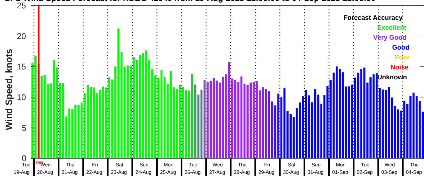
GFS Wind Speed Forecast for NDBC 41040 from 19-Aug-2025 21:00:00 to 04-Sep-2025 21:00:00
