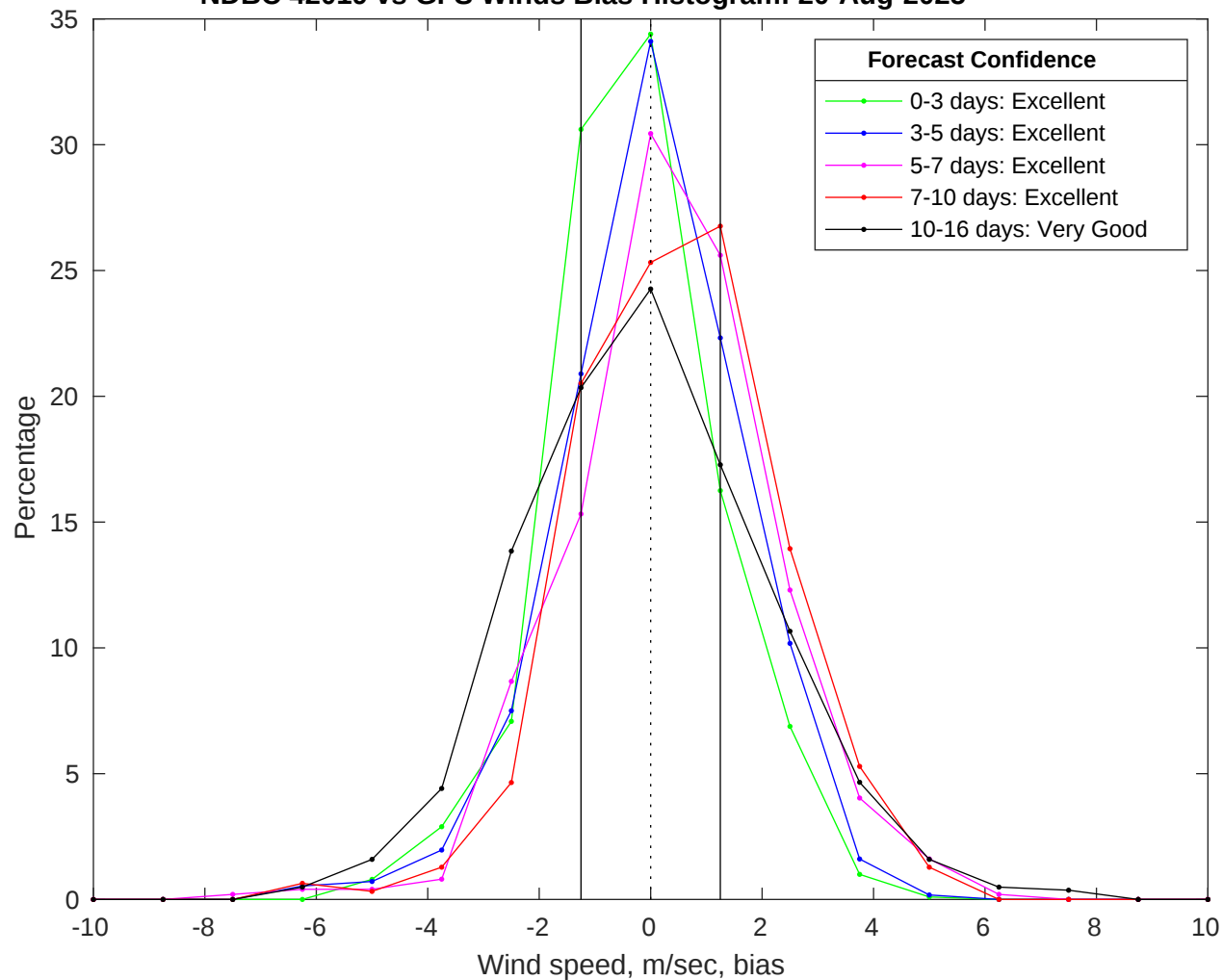
NDBC 42019 vs GFS Winds Bias Histogram: 20-Aug-2025
