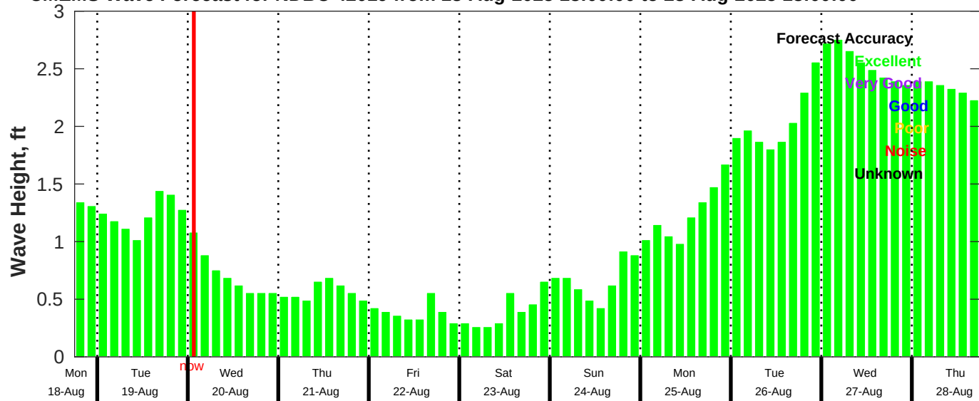
CMEMS Wave Forecast for NDBC 42019 from 18-Aug-2025 18:00:00 to 28-Aug-2025 18:00:00
