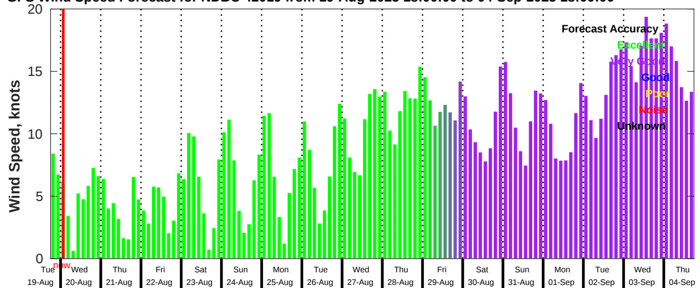
GFS Wind Speed Forecast for NDBC 42019 from 19-Aug-2025 18:00:00 to 04-Sep-2025 18:00:00
