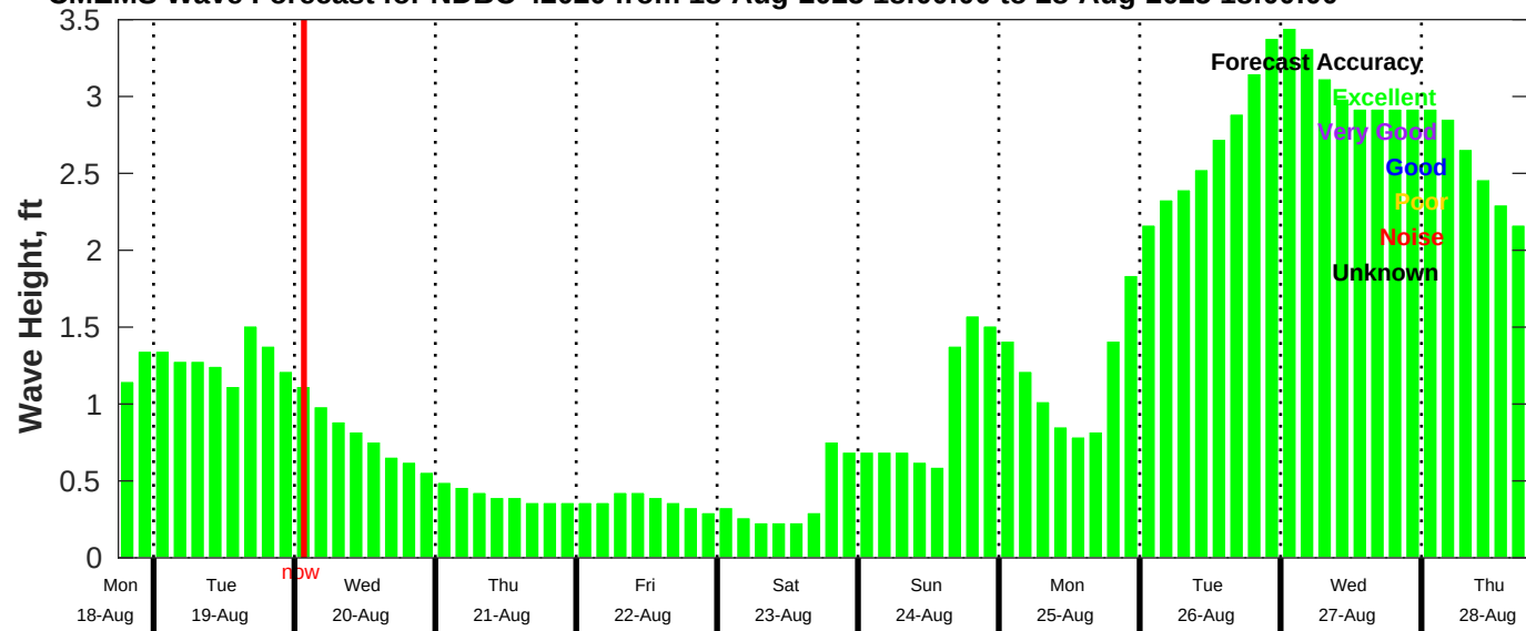
CMEMS Wave Forecast for NDBC 42020 from 18-Aug-2025 18:00:00 to 28-Aug-2025 18:00:00
