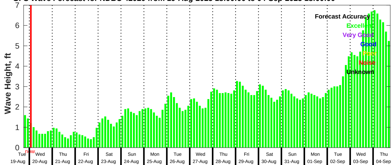
GFS Wave Forecast for NDBC 42020 from 19-Aug-2025 18:00:00 to 04-Sep-2025 18:00:00
