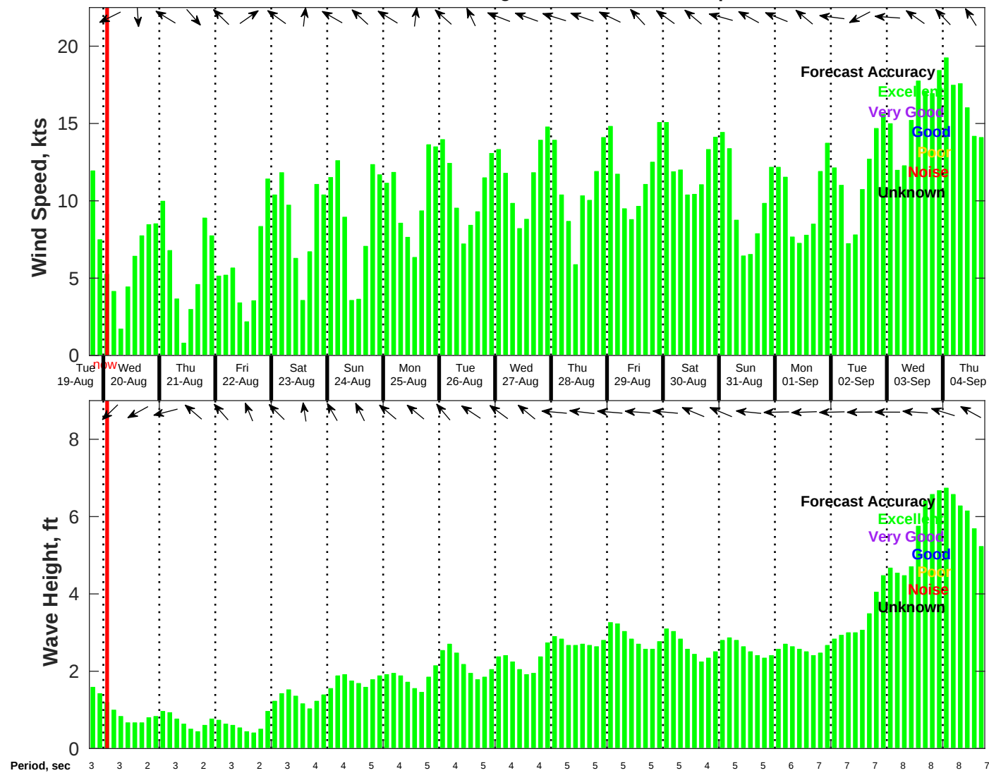
Wind & Wave Forecast for NDBC 42020 from 19-Aug-2025 18:00:00 to 04-Sep-2025 18:00:00
