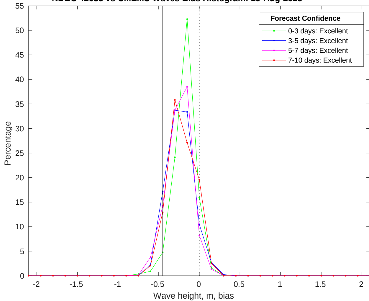
NDBC 42035 vs CMEMS Waves Bias Histogram: 19-Aug-2025
