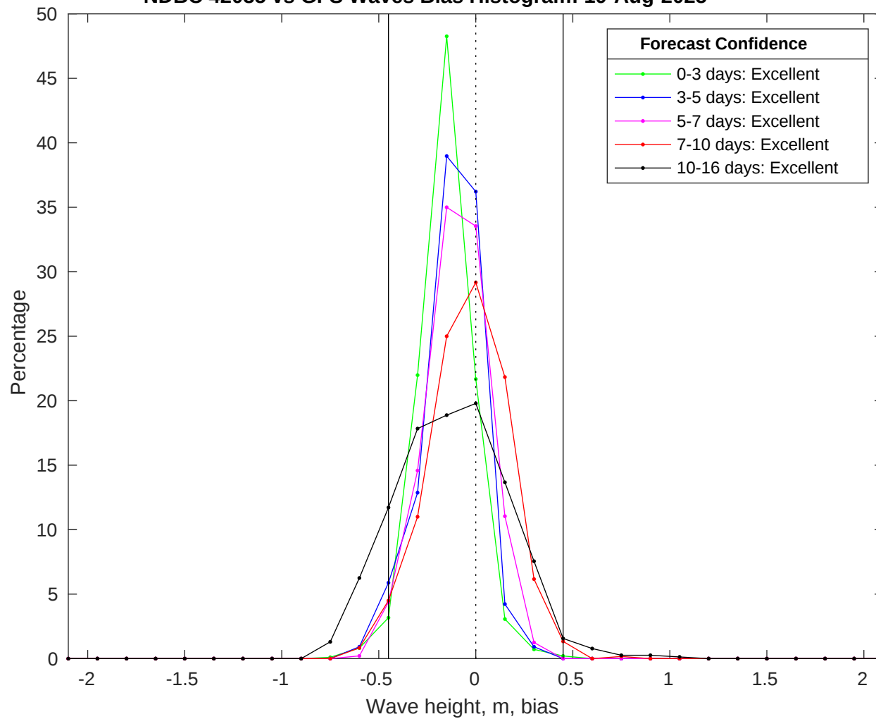
NDBC 42035 vs GFS Waves Bias Histogram: 19-Aug-2025
