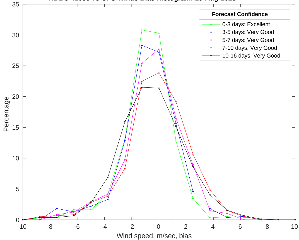
NDBC 42035 vs GFS Winds Bias Histogram: 19-Aug-2025
