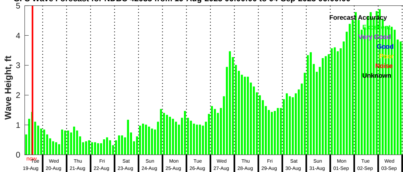
GFS Wave Forecast for NDBC 42035 from 19-Aug-2025 06:00:00 to 04-Sep-2025 06:00:00
