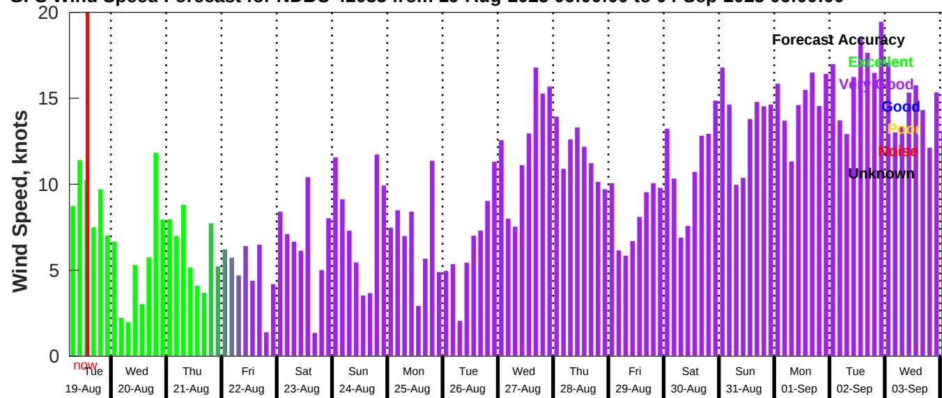
GFS Wind Speed Forecast for NDBC 42035 from 19-Aug-2025 06:00:00 to 04-Sep-2025 06:00:00
