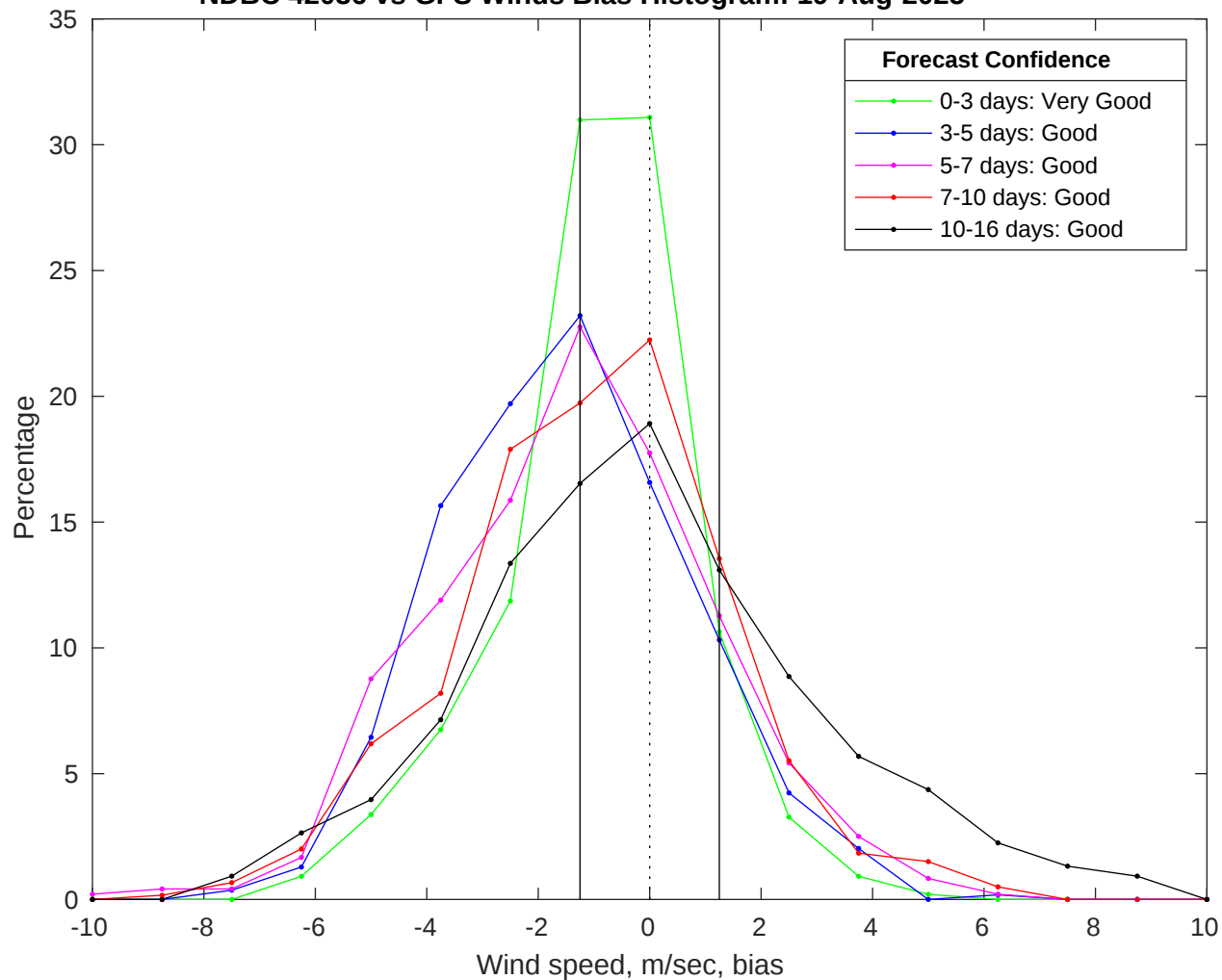
NDBC 42036 vs GFS Winds Bias Histogram: 19-Aug-2025
