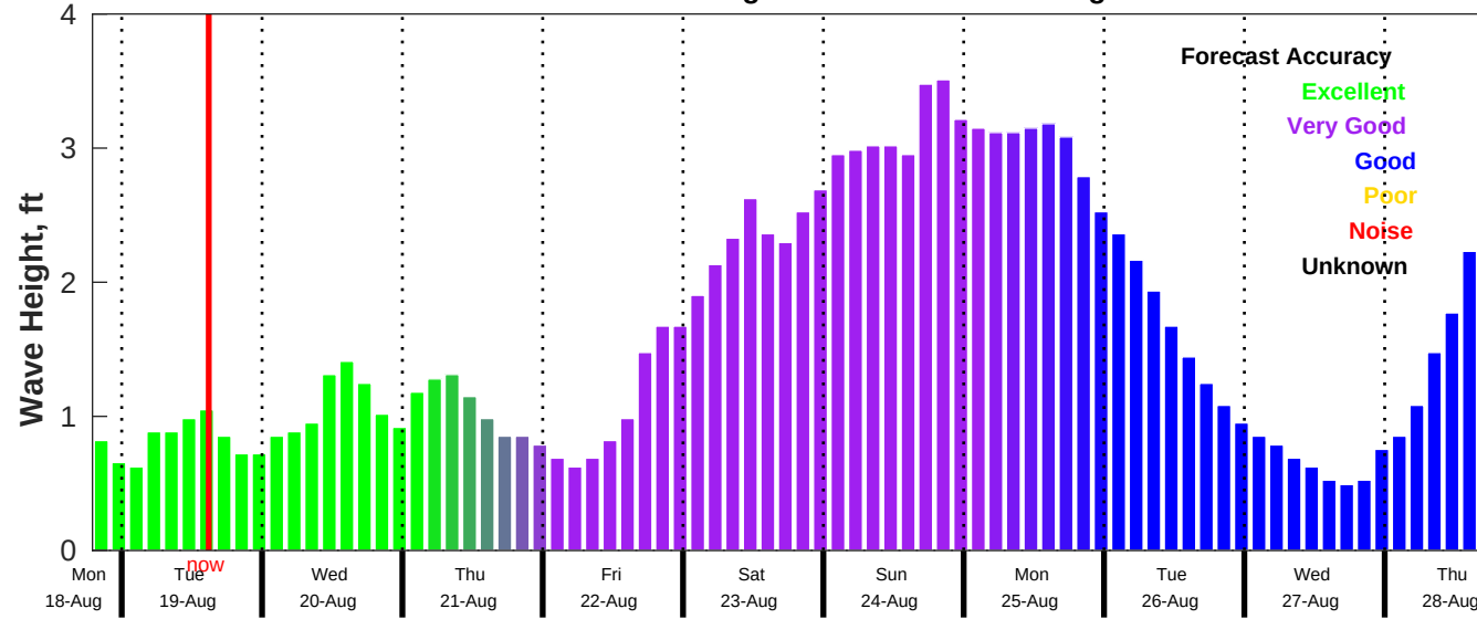
CMEMS Wave Forecast for NDBC 42036 from 18-Aug-2025 19:00:00 to 28-Aug-2025 19:00:00
