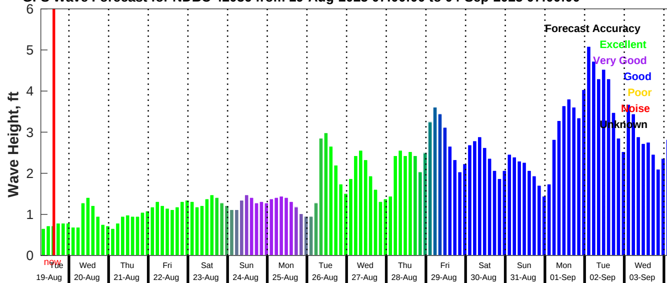
GFS Wave Forecast for NDBC 42036 from 19-Aug-2025 07:00:00 to 04-Sep-2025 07:00:00
