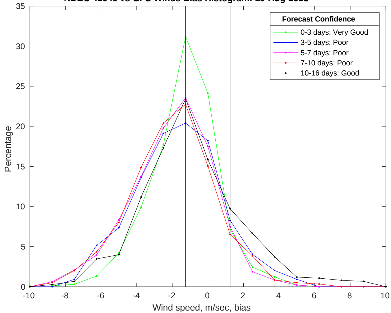
NDBC 42040 vs GFS Winds Bias Histogram: 19-Aug-2025
