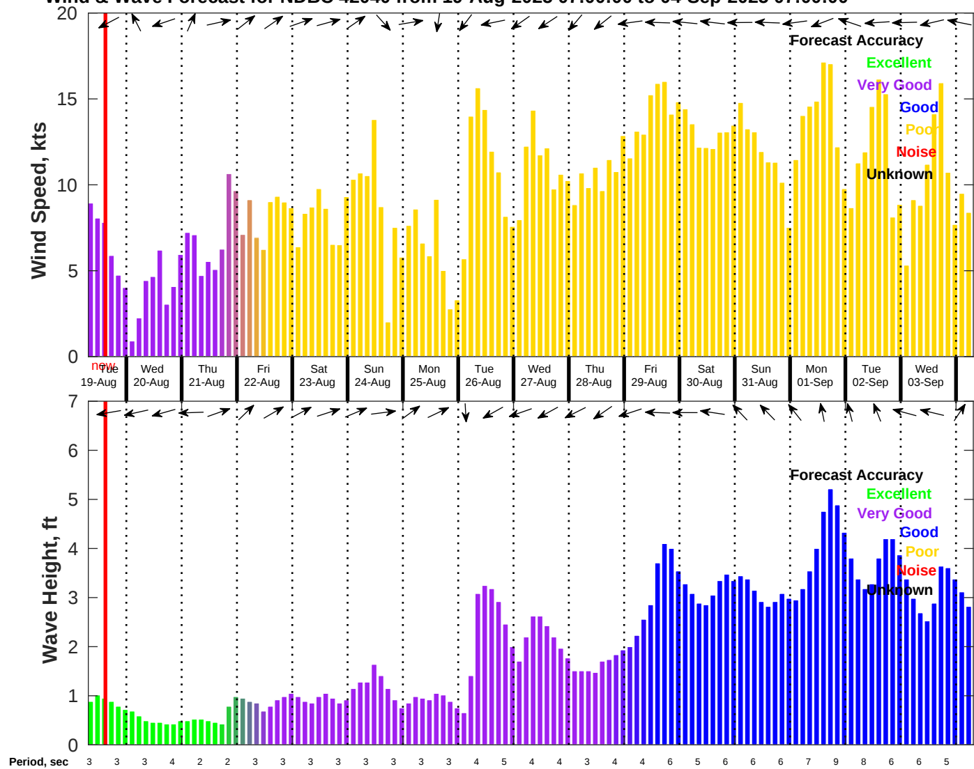
Wind & Wave Forecast for NDBC 42040 from 19-Aug-2025 07:00:00 to 04-Sep-2025 07:00:00
