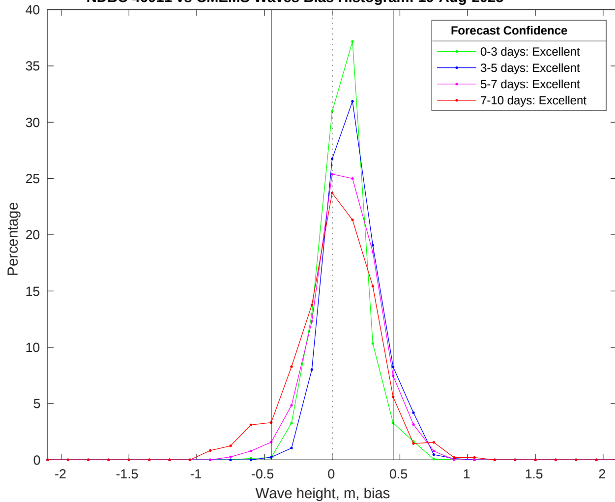
NDBC 46011 vs CMEMS Waves Bias Histogram: 19-Aug-2025
