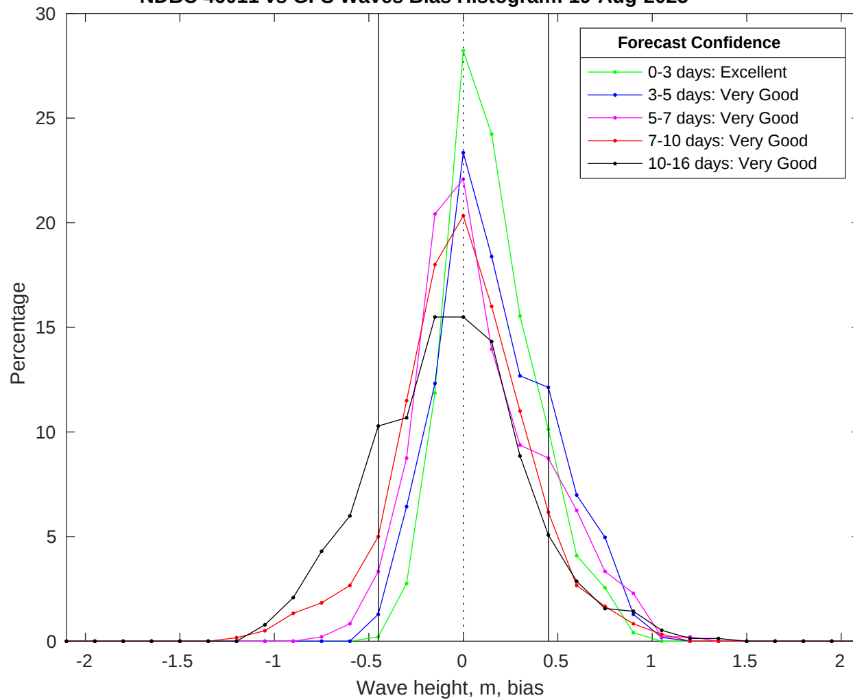
NDBC 46011 vs GFS Waves Bias Histogram: 19-Aug-2025
