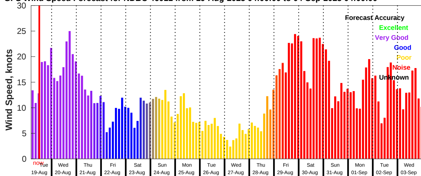
GFS Wind Speed Forecast for NDBC 46011 from 19-Aug-2025 04:00:00 to 04-Sep-2025 04:00:00
